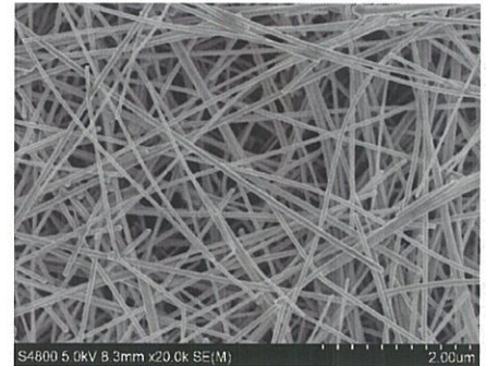
SEM image of CST-NW-S40
